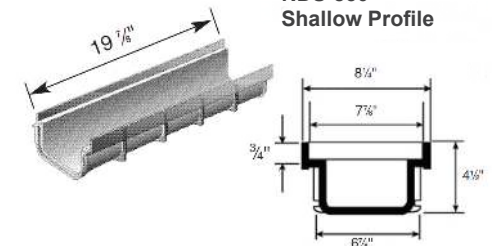
NDS-830 Shallow Profile
