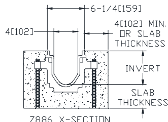
Z886 X-SECTION
