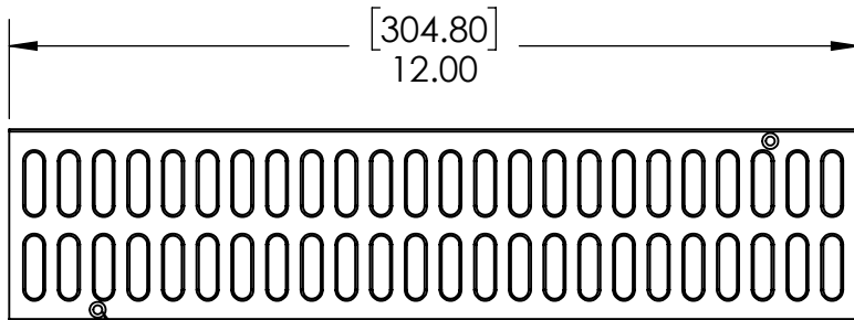
(2) COUNTER-SUNK HOLES DESIGNED FOR #4 HARDWARE
