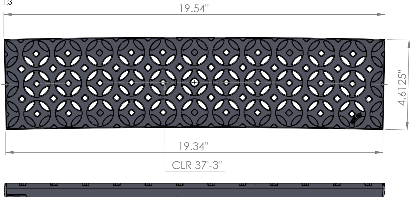
Top View Scale 1:3
