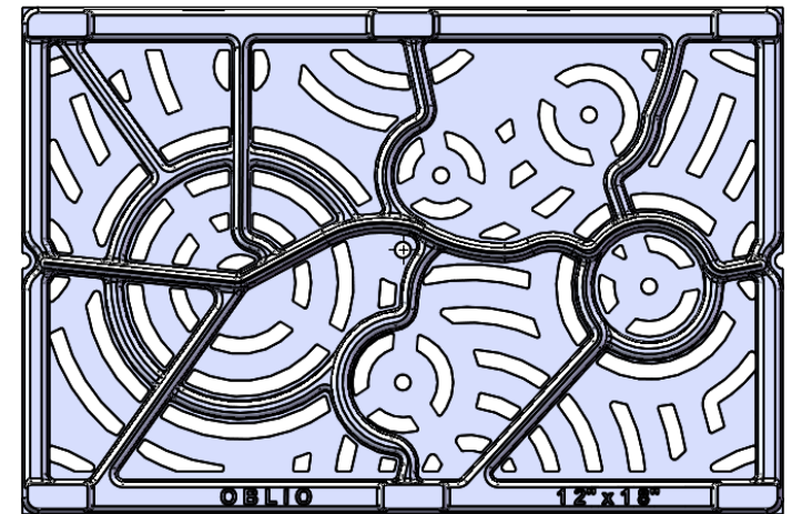
BACK scale 1:5
