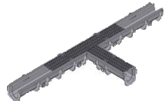
Tee Fabrication
