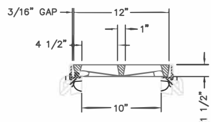
R-4999-CX TYPE "A" GRATE WITH TYPE "B" FRAME TYPICAL SECTION
