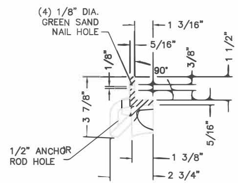
FRAME SECTION SCALE 1:2
