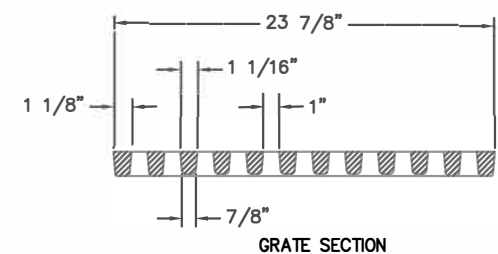
GRATE SECTION
